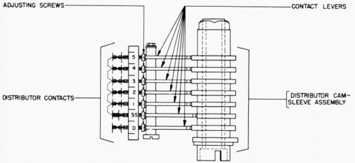
BOTTOM VIEW FIGURE 25
