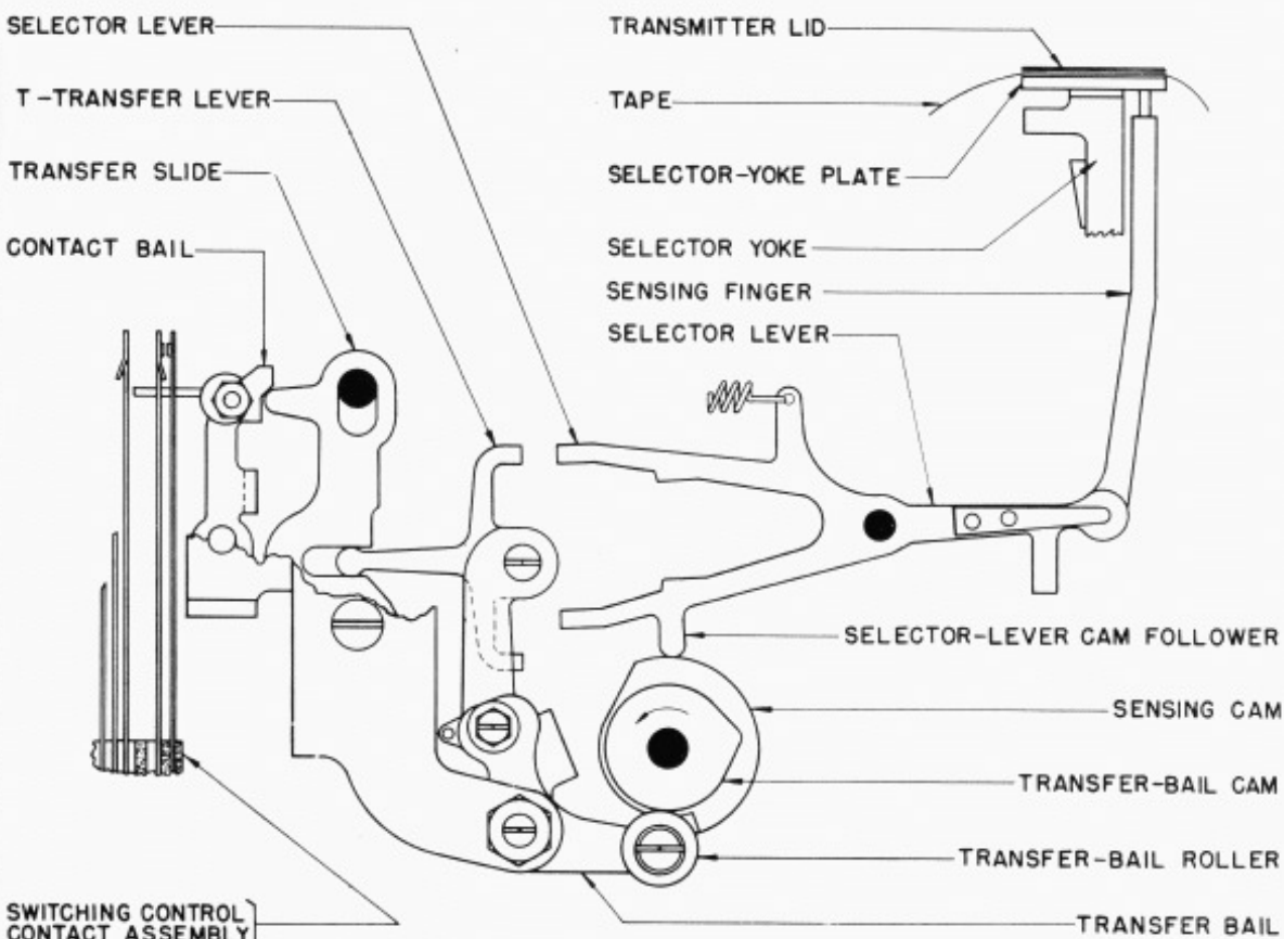
FRONT VIEW FIGURE 23
