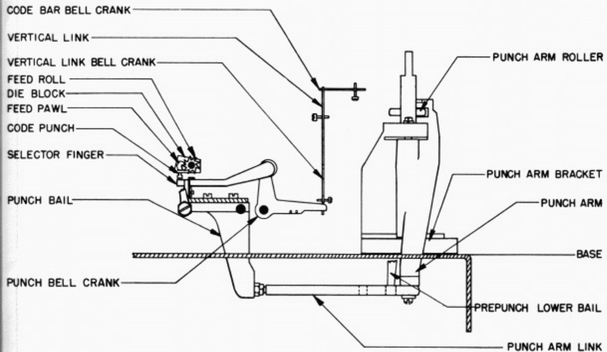
FRONT VIEW FIGURE 10
