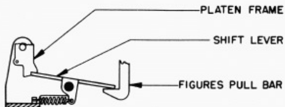
FRONT VIEW FIGURE 17
