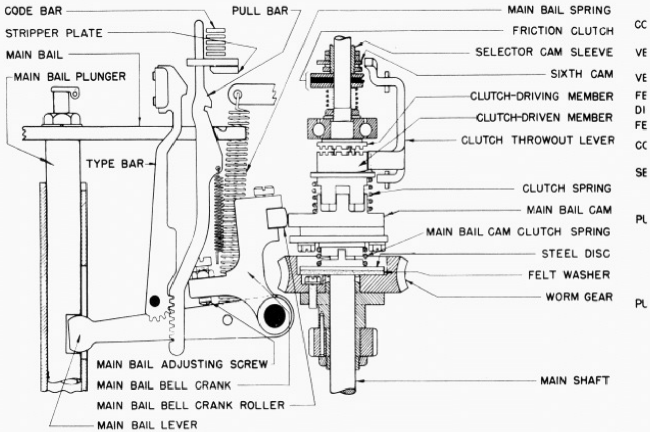
RIGHT SIDE VIEW FIGURE 7
