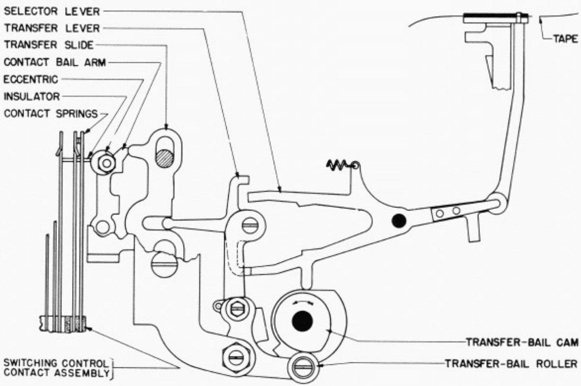
FRONT VIEW FIGURE 24
