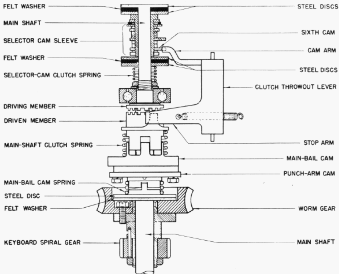
RIGHT SIDE VIEW FIGURE 4
